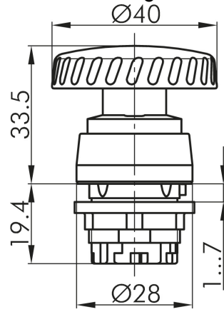
Dimensional drawing:
